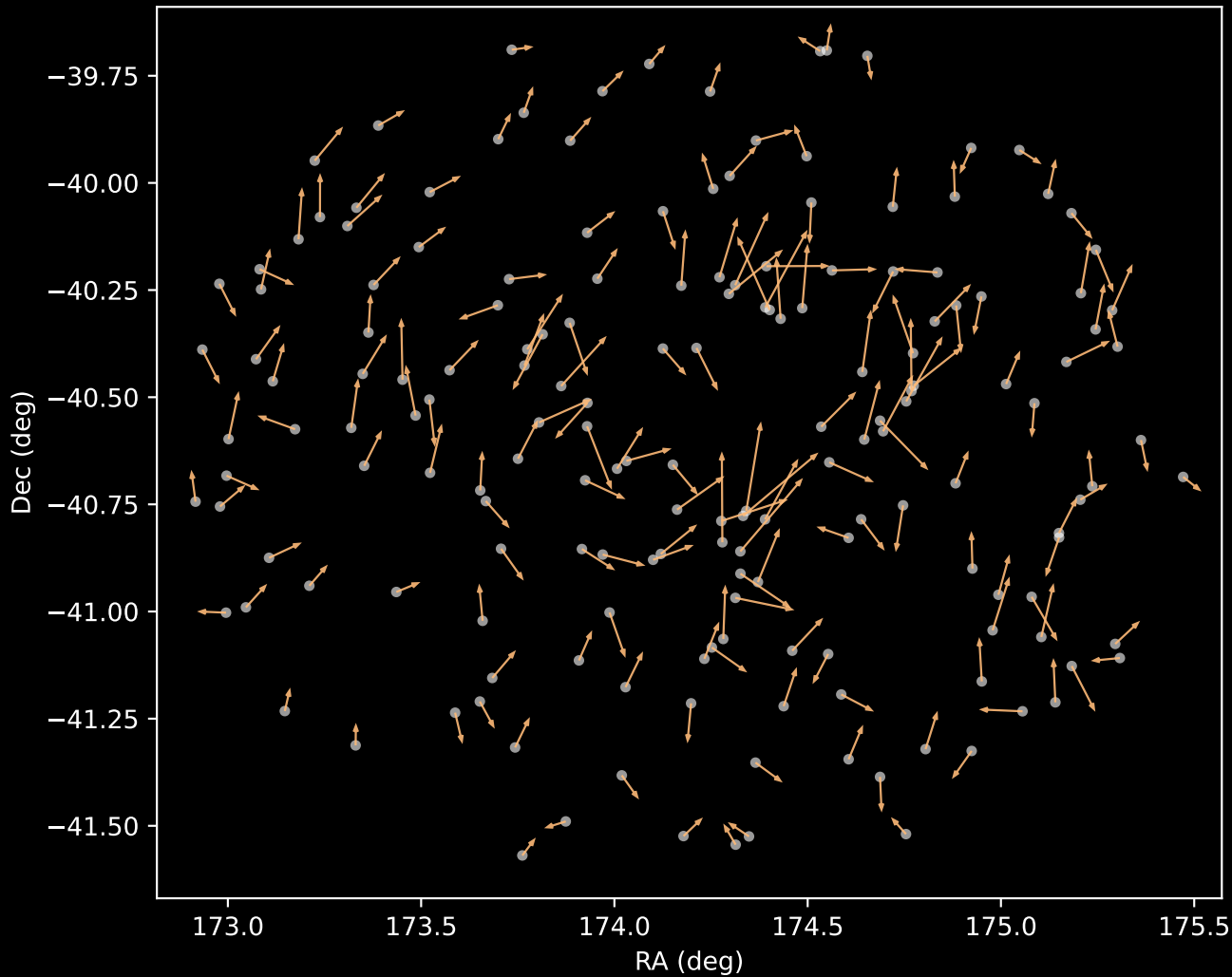
GALAH DR4 Cluster 3 Proper Motion Vectors (n=176)
