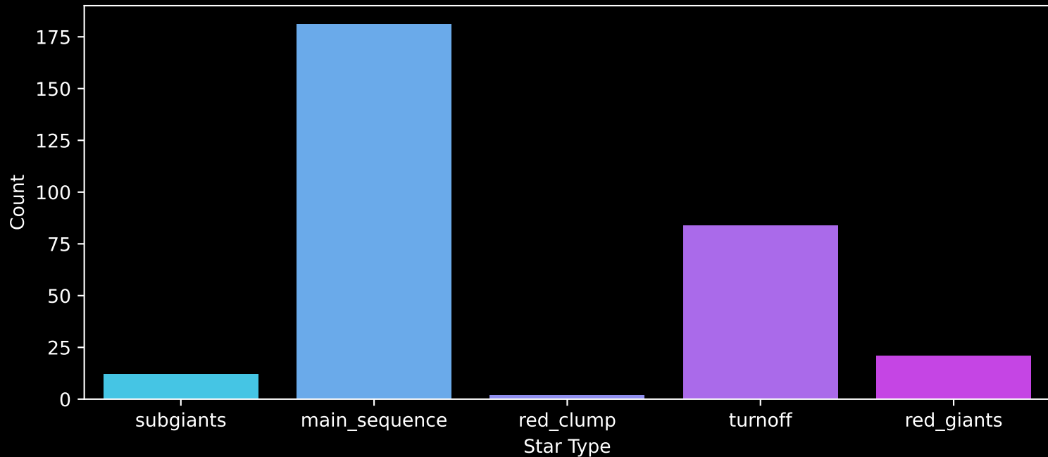
GALAH DR4 Field: [337] Count plot of Star Type
