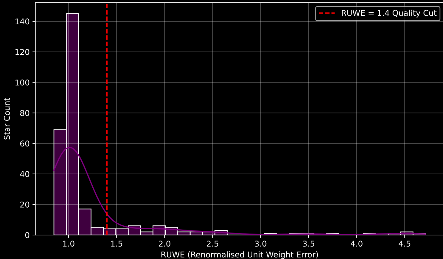
GALAH DR4 Field [337] RUWE Distribution (n= 281)
